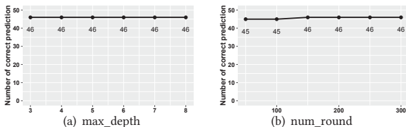
Figure 4: Impact of parameters on PTP
