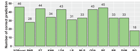
Figure 5: Effectiveness of machine learning algorithms
