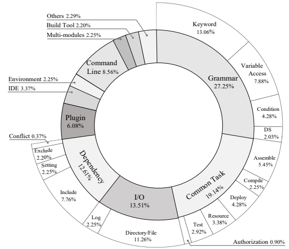
Figure 3: Topics in how-to build issues
