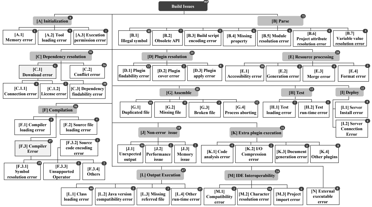
Figure 4: Taxonomy of symptoms in build issues
