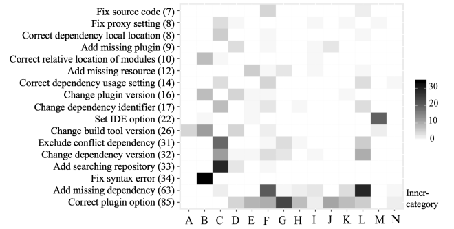
Figure 5: Distribution of fix patterns on inner-categories
