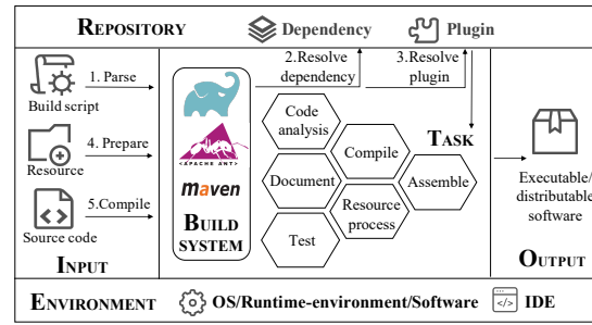
Figure 1: Build workflow
